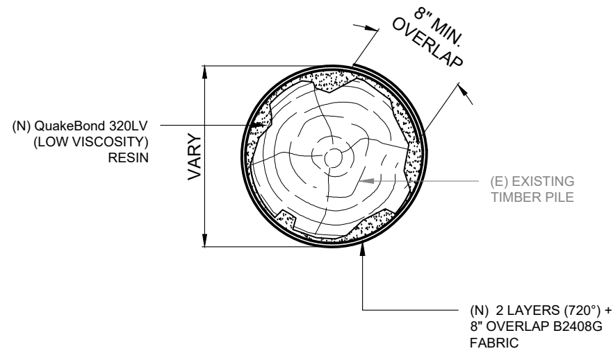
TIMBER PILE REPAIR CROSS SECTION 2 SCALE: 1=1/2"=1'-0" S-01
