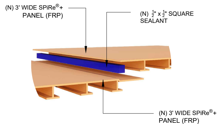
TYPICAL SPIRe®+ PANEL OVERLAP DETAIL
