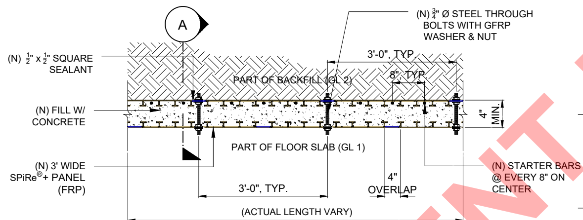
NEW RETAINING WALL SPIRe®+ DETAILS TYPICAL PARTIAL PLAN SCALE: NTS.
