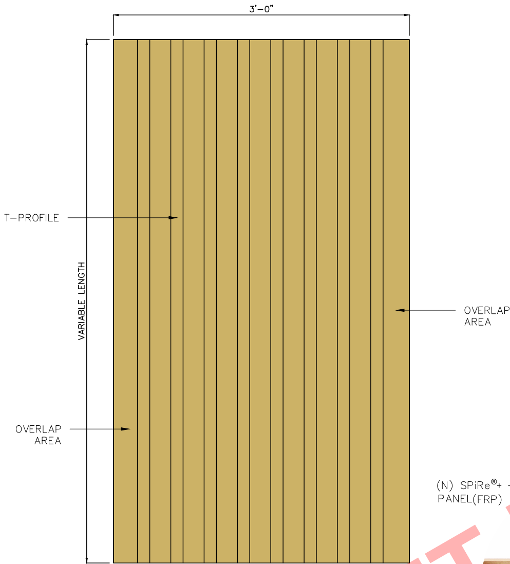
TYPICAL SPIRe ® + PANEL ELEVATION SCALE: 1"=1'-0"
