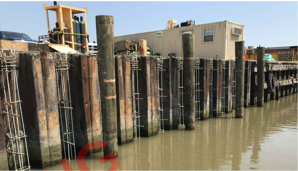
EXISTING SEAWALL
