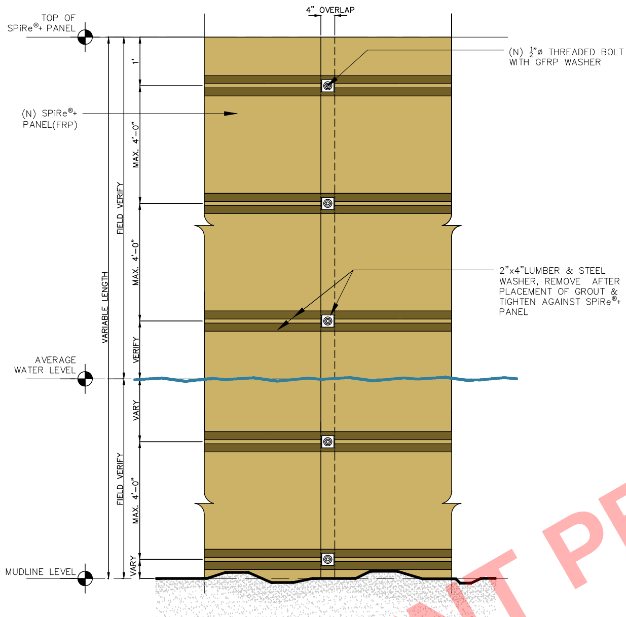
TYPICAL STRONGBACK ELEVATION
