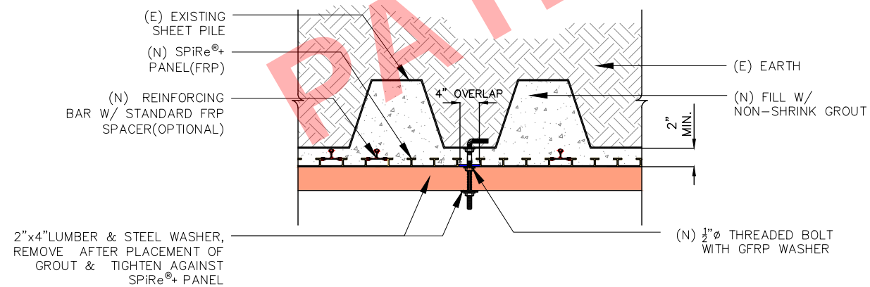
TYPICAL STRONGBACK PLAN VIEW
