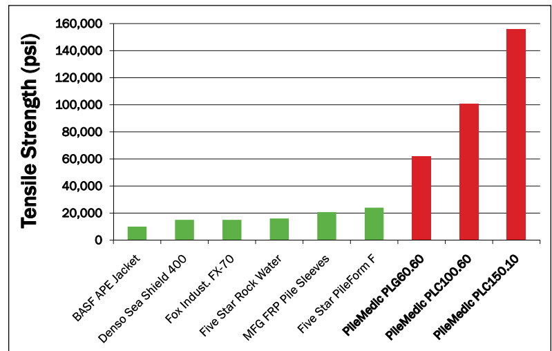
Fig. 3: Comparison of Tensile Strength of PileMedic™ with Conventional Jackets (Data compiled from information obtained from each company's website and literature.)
