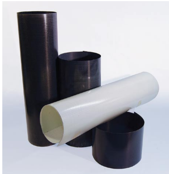
Fig. 2: Sample rolls of PileMedic™ carbon and glass laminates
