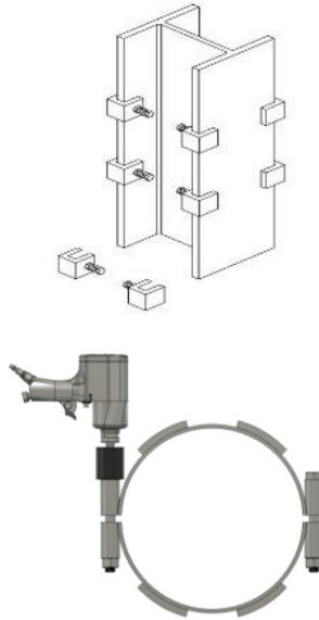
Fig. 4. ShearClamp™ used on H-piles and ShearWrap™ steel bands that are torqued around circular steel piles.
