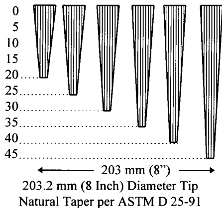
Figure 6—Natural Taper Round Timber Piling
